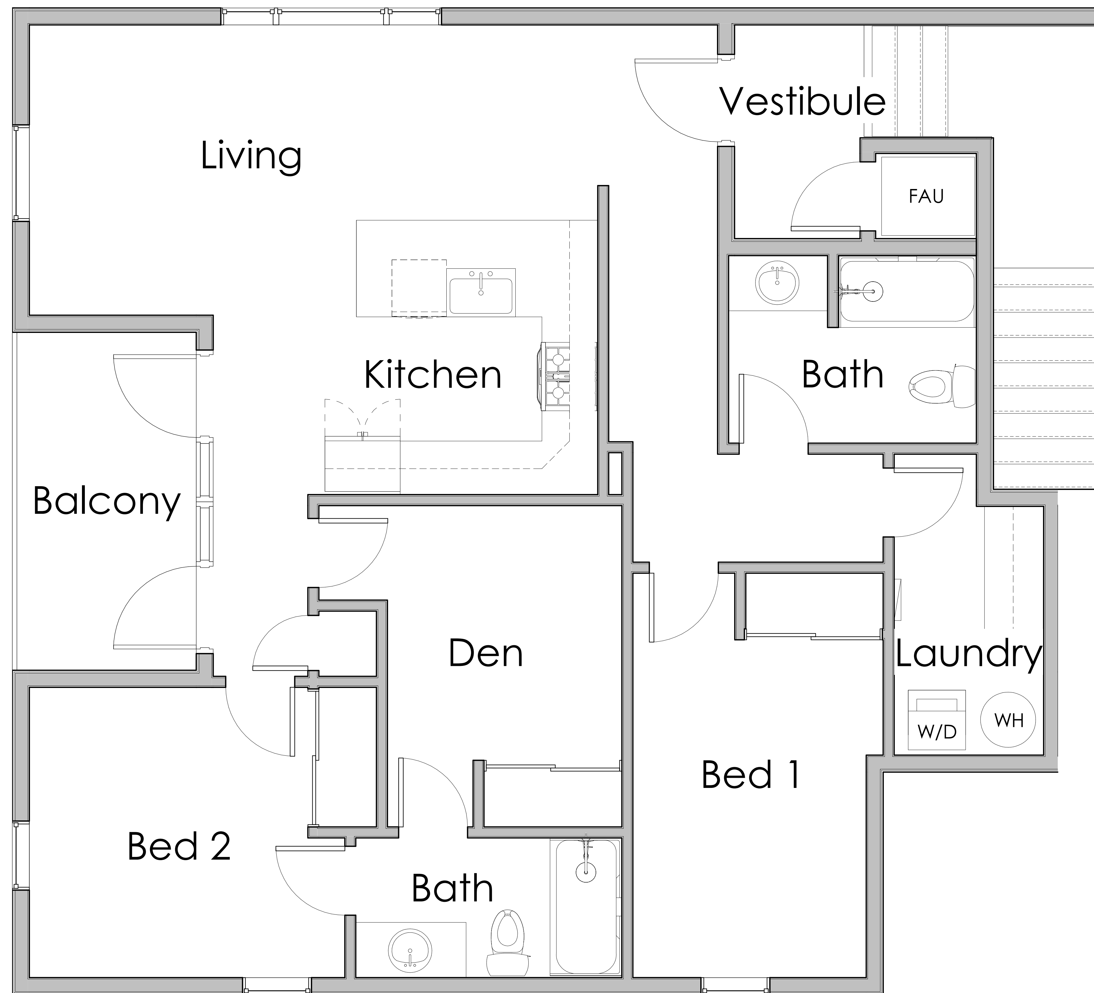
Apt. 2A Approx. 1096 Square Feet
